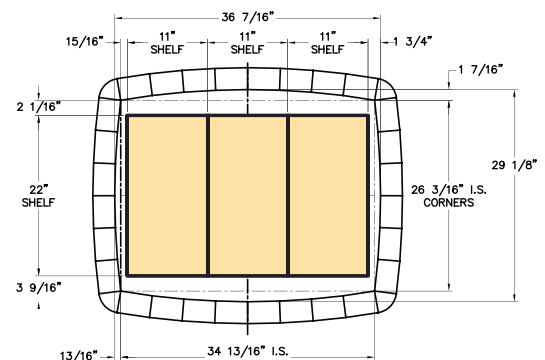
An T2327-D is shown with three sections. The control panel is mounted on the right side of the kiln. The handheld DynaTrol can be mounted on the wall (a 4 foot cord is included).
